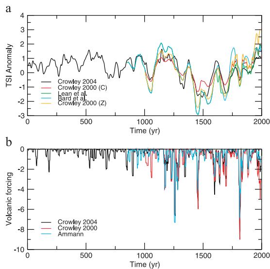
Figure 1. (a) Time variations of solar irradiance at the top of the atmosphere following the reconstructions of Lean et al. [1995] (green), Bard et al. [2000] (turquoise), Crowley -2004 (black, updated from Crowley et al. [2003]) and two scalings derived from Crowley [2000] used in the experiments of group C (red) and Z (orange), respectively. (b) Time variations of volcanic forcing scaled as an effective change in solar irradiance for comparison with (a), following the reconstructions of Crowley [2000] (red), Crowley -2004 (updated from Crowley et al. [2003]) (black) and Ammann (as described by Jones and Mann [2004], turquoise). A 10-year running mean has been applied to the time series in order to highlight low frequency variations.
