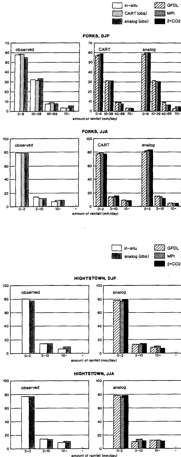
FIG. 11. Daily rainfall ( \text{mm day}^{-1} ) probability distribution (percent) as observed and generated by the CART and ANALOG methods from the NMC analysis and from different model runs in winter (DJF) and summer (JJA): (a) Forks (Pacific sector); (b) Hightstown (Atlantic sector).
