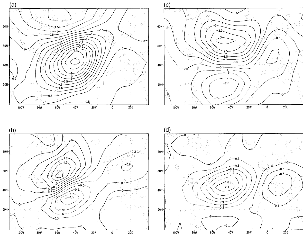
FIG. 1. First two pairs of CCA patterns of anomalous monthly \overline{\Psi}_{850} (units: 10^6 \text{ m}^2 \text{ s}^{-1} ) (upper) and anomalous monthly \overline{v'T'} at 750 hPa (units: \text{K m s}^{-1} ) (lower) in the North Atlantic sector derived from 2880 winter months simulated in the control run. (left) The first pair with a correlation of 0.85; they represent 29% of the \overline{\Psi}_{850} variance and 17% of the \overline{v'T'} variance. (right) The second pair with a correlation of 0.74 and 17% and 15% described variances.
