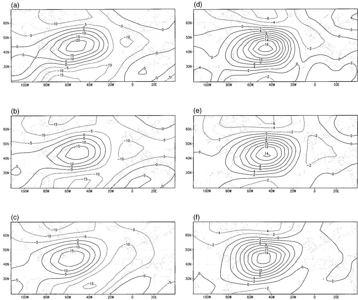
FIG. 4. An example of the anomalous monthly mean streamfunction (the long-term mean of the control run is subtracted; units, 10^6 \text{ m}^2 \text{ s}^{-1} ) simulated in the Eemian run and its analogue derived from the control run library; (left) 300-hPa and (right) 850-hPa streamfunction anomaly; (top) Eemian state, untruncated; (middle) Eemian state, truncated by the first 25 EOFs (search for a minimum in the truncated space); (bottom) control state, truncated by the first 25 EOFs. The \overline{v'T'} fields and \overline{\Psi} fields belonging to the Eemian mean state and to the control run analogue are shown in Fig. 5.
